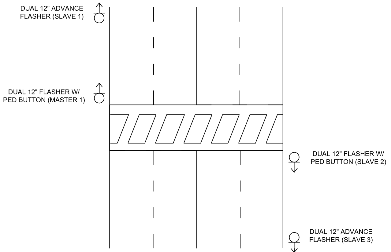
FIGURE 1. SOLAR PED-X CROSSWALK FLASHER SYSTEM WITH ADVANCE FLASHERS
